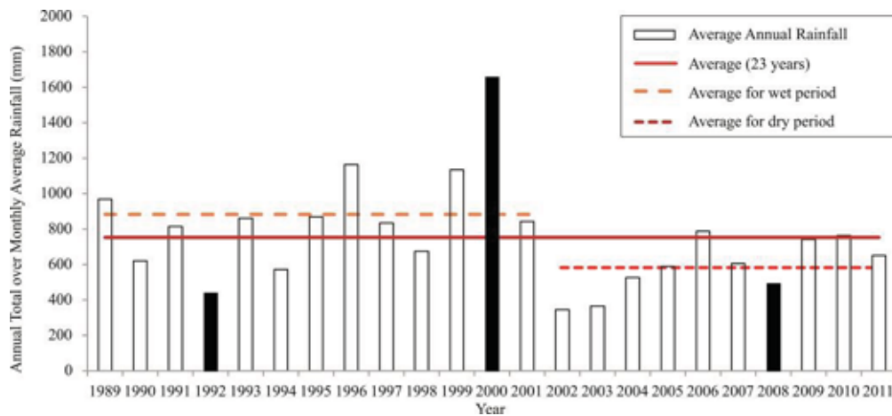
Figure 2. Average annual rainfall highlighting (in black) the wet year (2000) and dry years (1992 and 2008).
