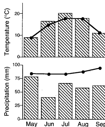
Figure 2. Climatic data for Rivière-du-Loup for the period May to September. Thirty-year normals (1961–1990) (lines) compared to the 1995 season (bars). Environment Canada (1993) and data from Ministère de l'Environnement et Faune du Québec for the summer 1995.
